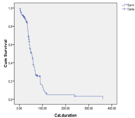
Survival Function
